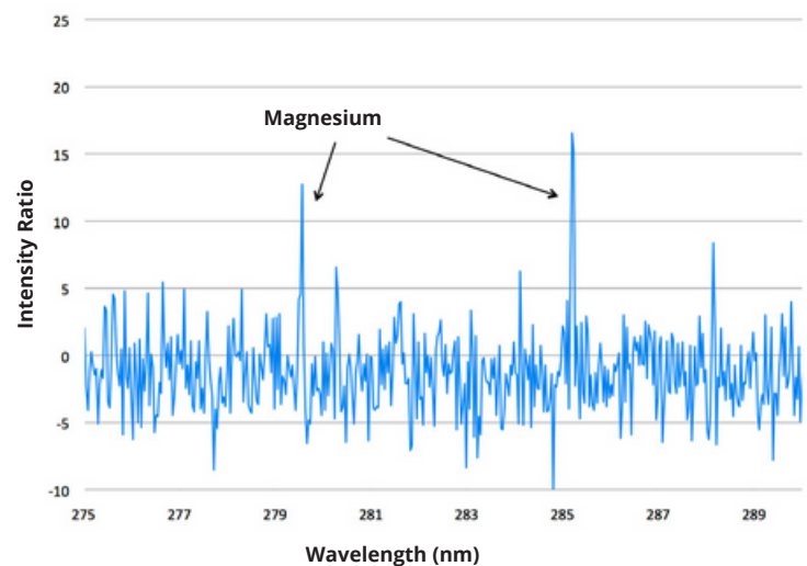
Figure 2: Spectrum for a 2 second test of a 1050 grade aluminum alloy containing 0.027% Mg.
