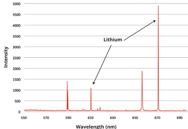
Figure 3: Spectrum from a 2 second test on aluminum alloy containing 1.86% lithium.
